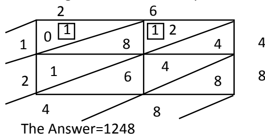
Figure: 2 Lattice multiplication
